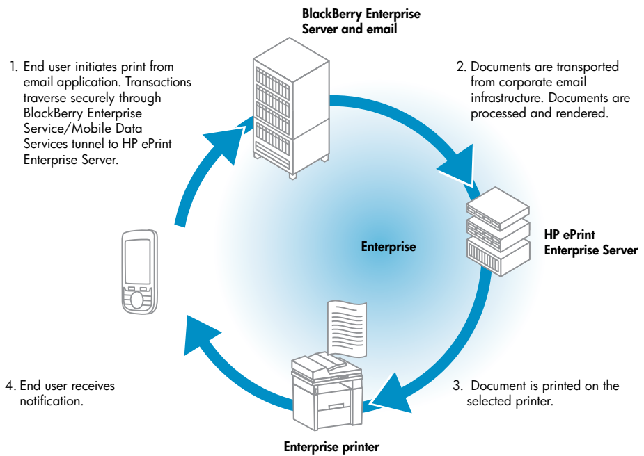
Figure 1. How the HP ePrint Enterprise solution works
